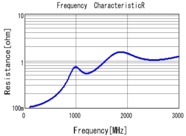
■ GRM31A5C2J331JW01 R DC0V, 25degC
