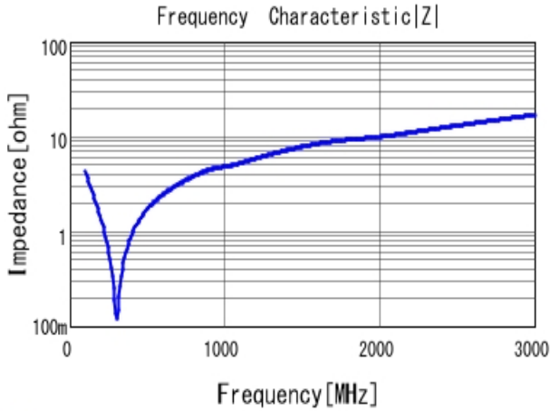
■ GRM31A5C2J331JW01 |Z| DC0V, 25degC
