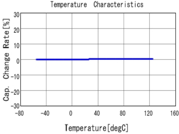
■ GRM31A5C2J331JW01 C-Temp. capchange, DCOV, AC1Vrms
