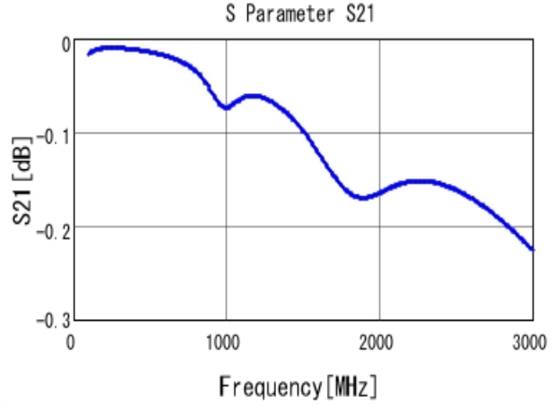
■ GRM31A5C2J331JW01 S21 DCOV, 25degC
