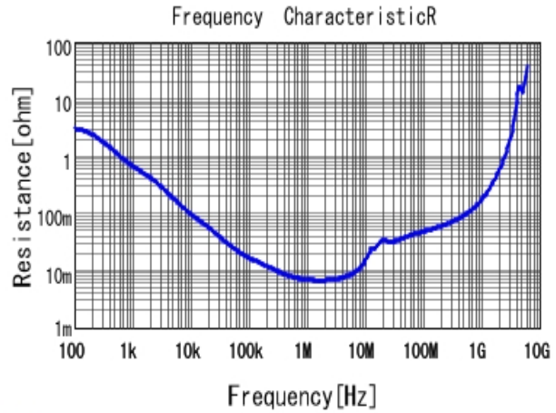
■ GRM319R71C105KAA3 R DCOV, 25degC
