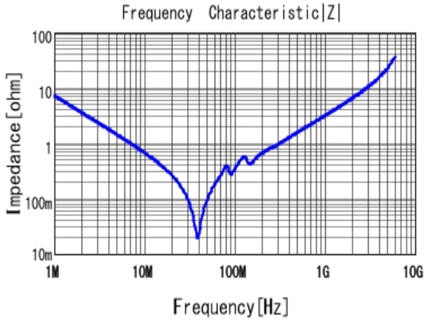
■ GRM3195C2A223JA01 |Z| DCOV, 25degC
