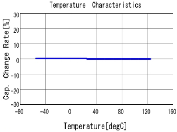
■ GRM3195C2A223JA01 C-Temp. capchange, DCOV, AC1Vrms
