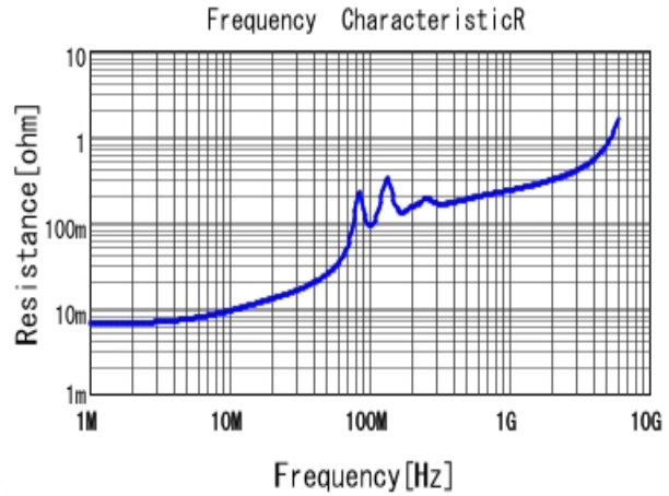
■ GRM3195C2A223JA01 R DCOV, 25degC
