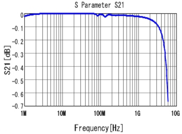
■ GRM3195C2A223JA01 S21 DCOV, 25degC
