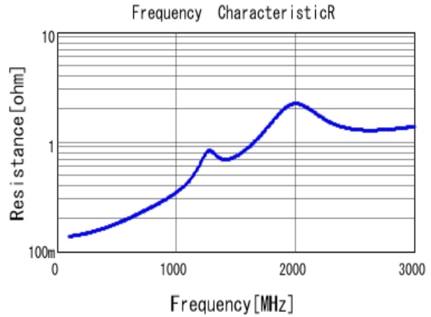
■ GRM21A7U2E121JW31 R DCOV, 25degC
