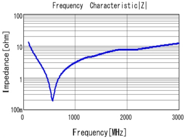
■ GRM21A7U2E121JW31 |Z| DCOV, 25degC
