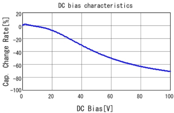
■ GRM188R72A223KAC4 C-DC bias capchange, 25.0degC, AC1.
