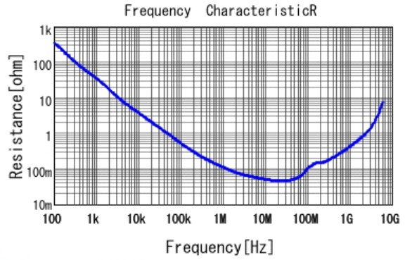
■ GRM188R72A223KAC4 R DCOV, 25degC
