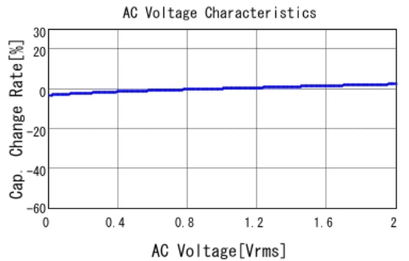
■ GRM188R72A223KAC4 C-AC Voltage capchange, DCOV, 25.0d
