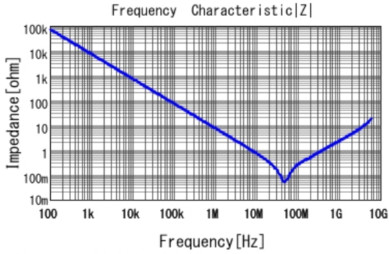
■ GRM188R72A223KAC4 |Z| DCOV, 25degC
