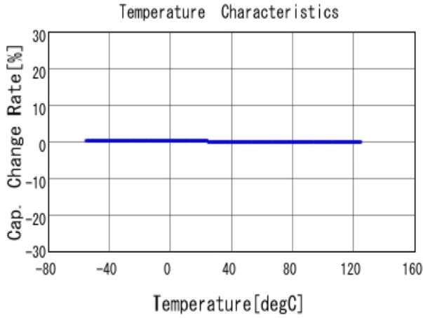
■ GRM1885C2A681JA01 C-Temp. capchange, DCOV, AC1Vrms
