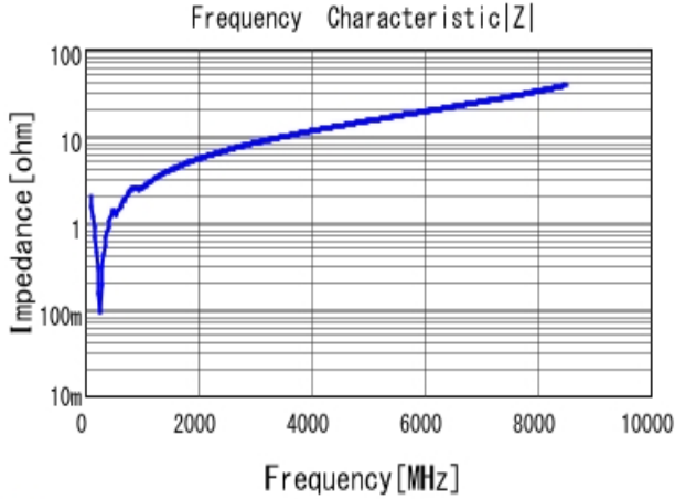
■ GRM1885C2A681JA01 |Z| DCOV, 25degC
