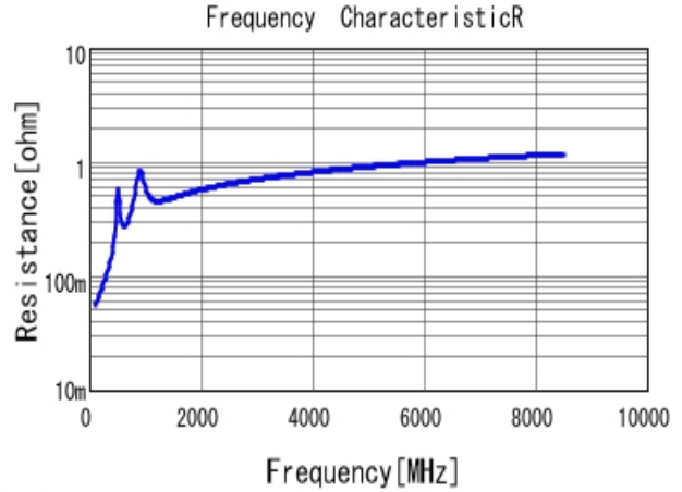
■ GRM1885C2A681JA01 R DCOV, 25degC
