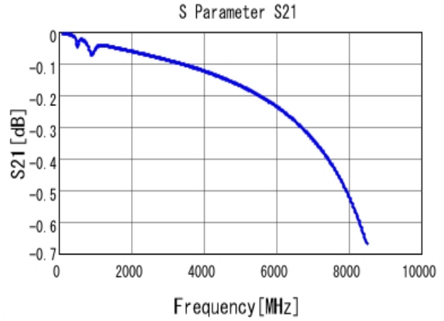
■ GRM1885C2A681JA01 S21 DCOV, 25degC
