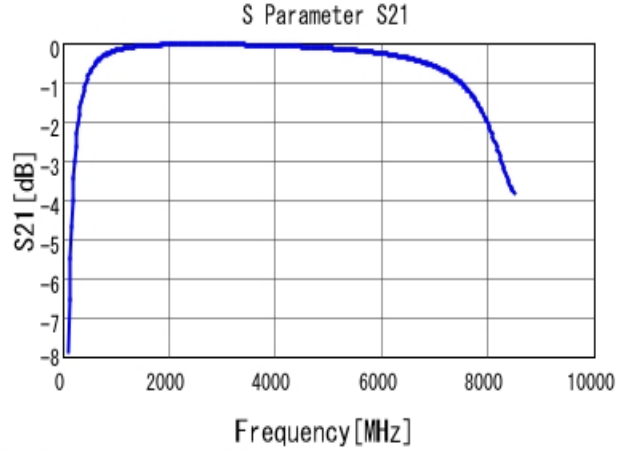
■ GRM1885C1H7R0DA01 S21 DCOV, 25degC
