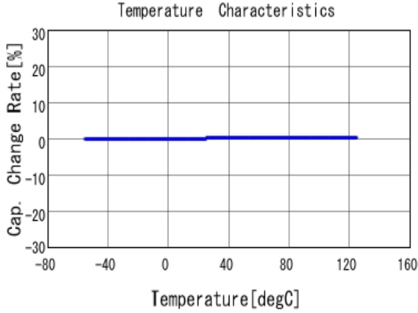
■ GRM1885C1H7R0DA01 C-Temp. capchange, DCOV, AC1Vrms
