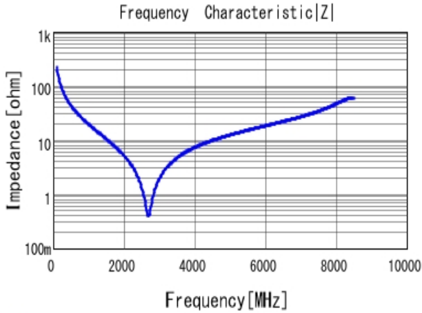
■ GRM1885C1H7R0DA01 |Z| DCOV, 25degC
