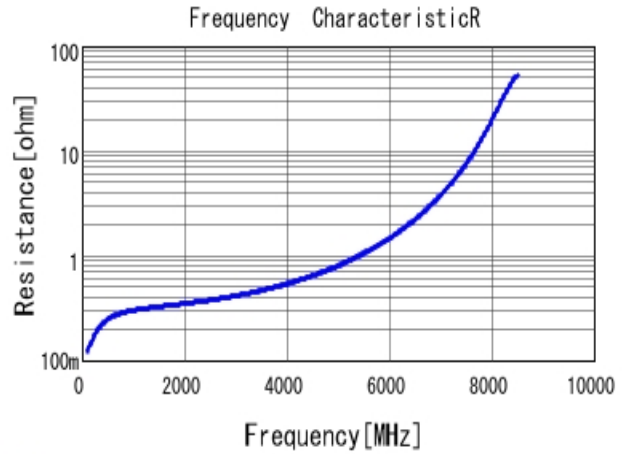
■ GRM1885C1H7R0DA01 R DCOV, 25degC
