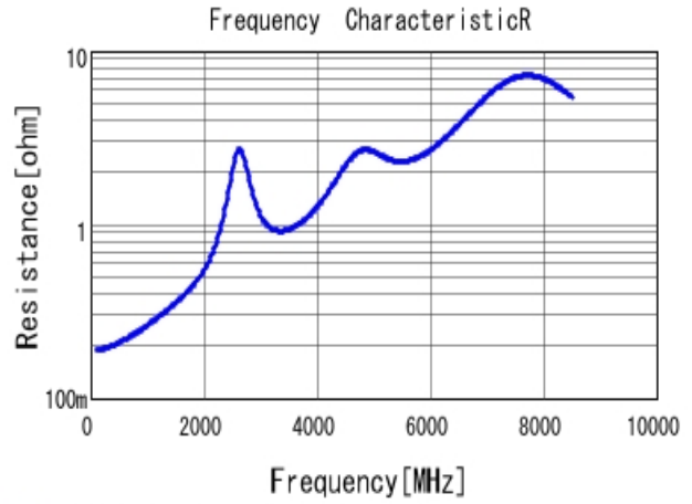
■ GRM1885C1H330GA01 R DC0V, 25degC
