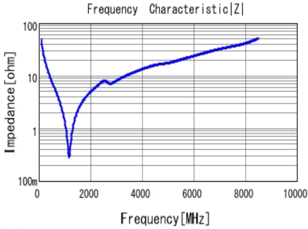
■ GRM1885C1H330GA01 |Z| DC0V, 25degC
