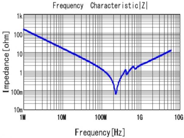
■ GRM1885C1E102JA01 |Z| DCOV, 25degC
