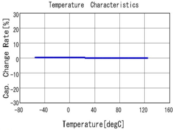
■ GRM1885C1E102JA01 C-Temp. capchange, DCOV, AC1Vrms
