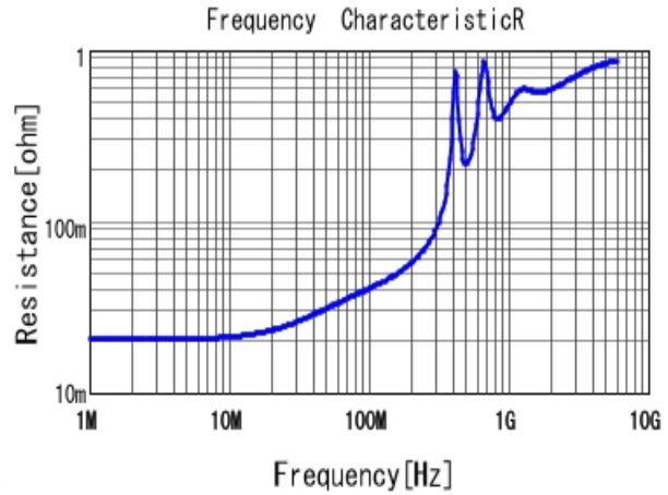
■ GRM1885C1E102JA01 R DCOV, 25degC
