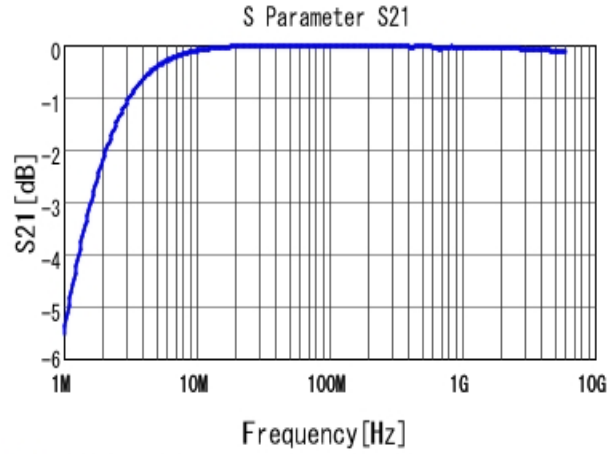
■ GRM1885C1E102JA01 S21 DCOV, 25degC
