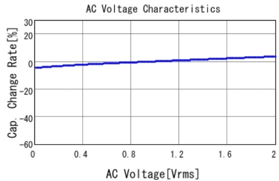
■ GRM155R71C333KA01 C-AC Voltage capchange, DCOV, 25.0d
