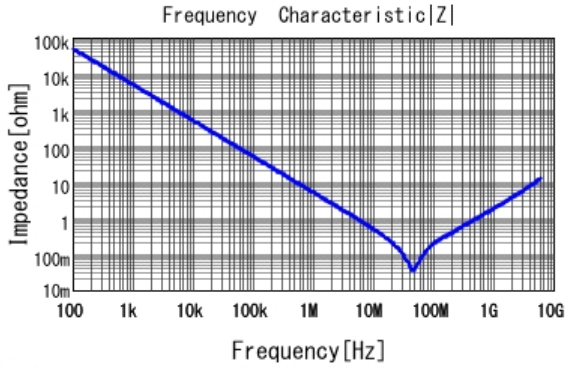
■ GRM155R71C333KA01 |Z| DCOV, 25degC
