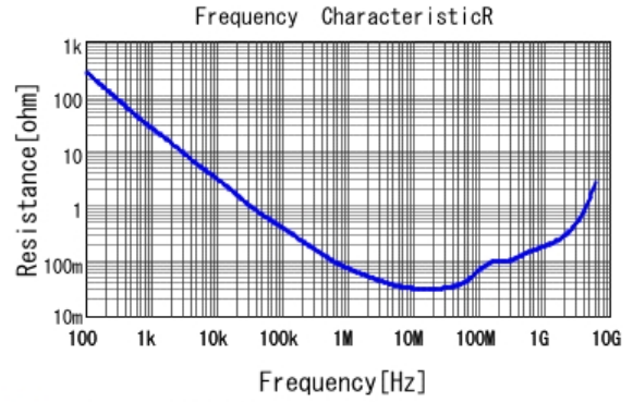
■ GRM155R71C333KA01 R DCOV, 25degC
