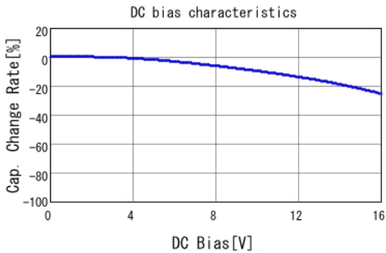
■ GRM155R71C333KA01 C-DC bias capchange, 25.0degC, AC1.
