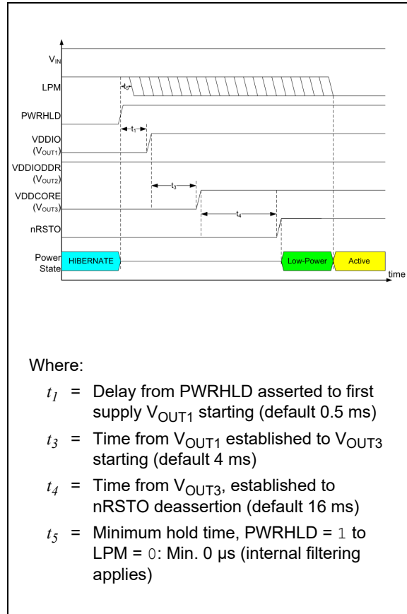
FIGURE 4-9: Start-up Sequence Exiting Hibernate Mode Timing Diagram.
