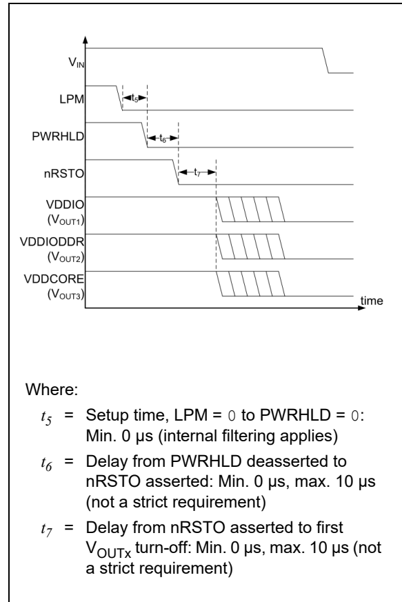
FIGURE 4-7: Power-Down (Shutdown) Sequence Timing Diagram.
