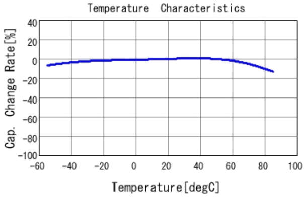
GRM155R60G475ME87 C-Temp. capchange, DC0.0V, AC0.2
