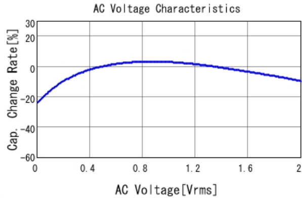
GRM155R60G475ME87 C-AC Voltage capchange, DCOV, 25
