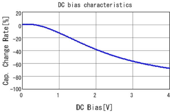
GRM155R60G475ME87 C-DC bias capchange, 25.0degC, A
