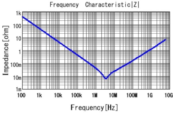
GRM155R60G475ME87 |Z| DCOV, 25degC
