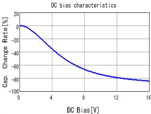
■ GRM155C81C225KE11 C-DC bias capchange, 25.0degC, AC1V
