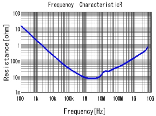
■ GRM155C81C225KE11 R DCOV, 25degC
