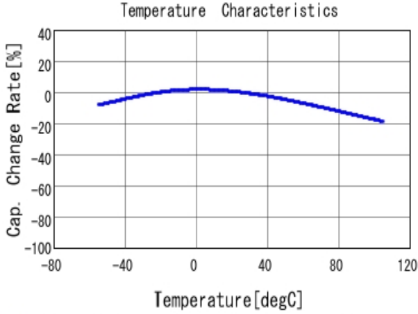
■ GRM155C81C225KE11 C-Temp. capchange, DC0.0V, AC0.2V rm
