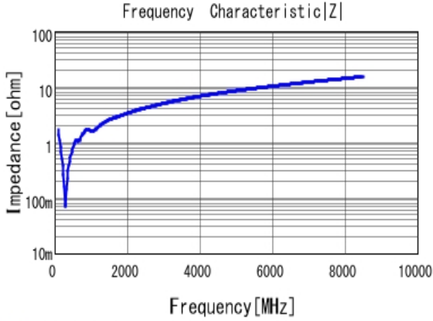
■ GRM1555C1H821JA01 |Z| DCOV, 25degC
