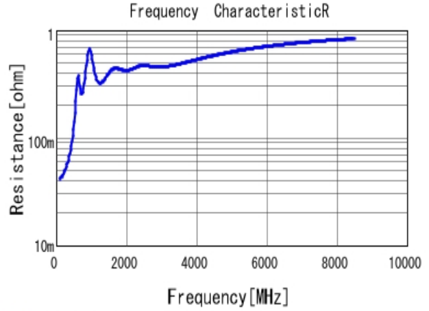
■ GRM1555C1H821JA01 R DCOV, 25degC
