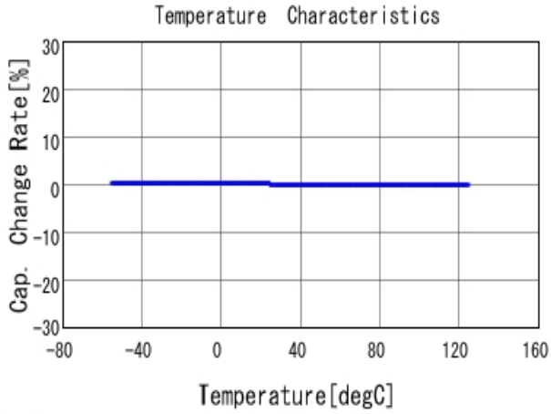
■ GRM1555C1H821JA01 C-Temp. capchange, DCOV, AC1Vrms
