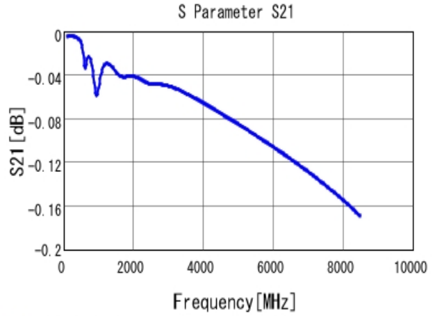
■ GRM1555C1H821JA01 S21 DCOV, 25degC
