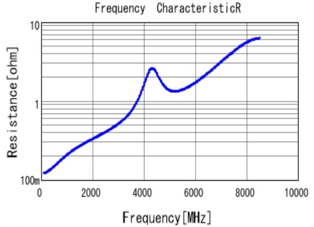
■ GRM1555C1E180JA01 R DCOV, 25degC
