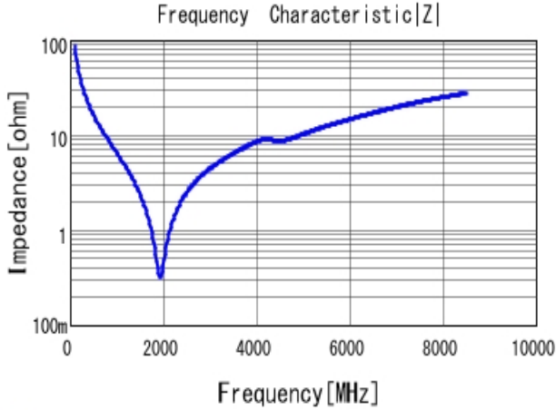
■ GRM1555C1E180JA01 |Z| DCOV, 25degC
