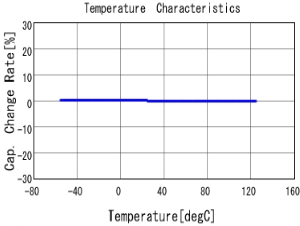
■ GRM1555C1E180JA01 C-Temp. capchange, DCOV, AC1Vrms
