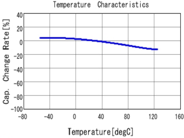
■ GRM033R70J103KA01 C-Temp. capchange, DCO. 0V, AC1.0V rm
