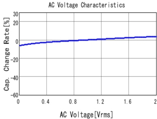
■ GRM033R70J103KA01 C-AC Voltage capchange, DCOV, 25.0d
