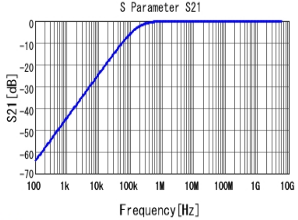
■ GRM033R70J103KA01 S21 DCOV, 25degC
