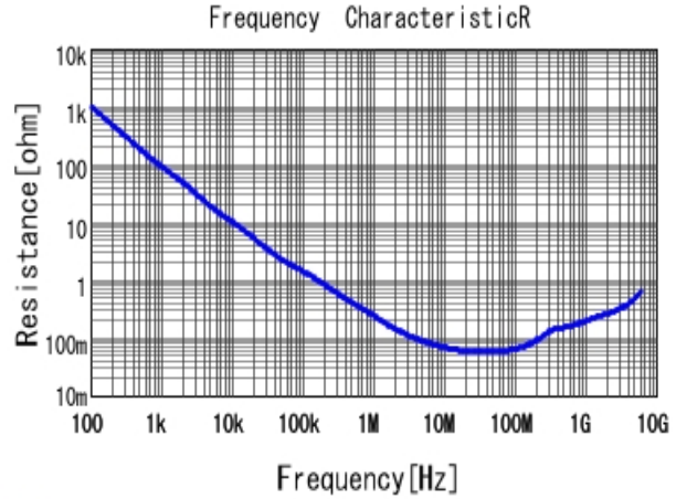
■ GRM033R70J103KA01 R DCOV, 25degC
