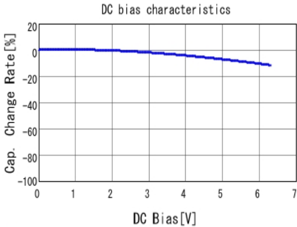
■ GRM033R70J103KA01 C-DC bias capchange, 25.0degC, AC1.
