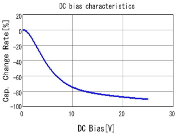
■ GRM033C81E104KE14 C-DC bias capchange, 25.0degC, AC1V
