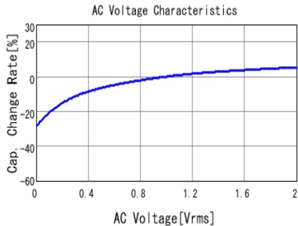
■ GRM033C81E104KE14 C-AC Voltage capchange, DCOV, 25.0d
