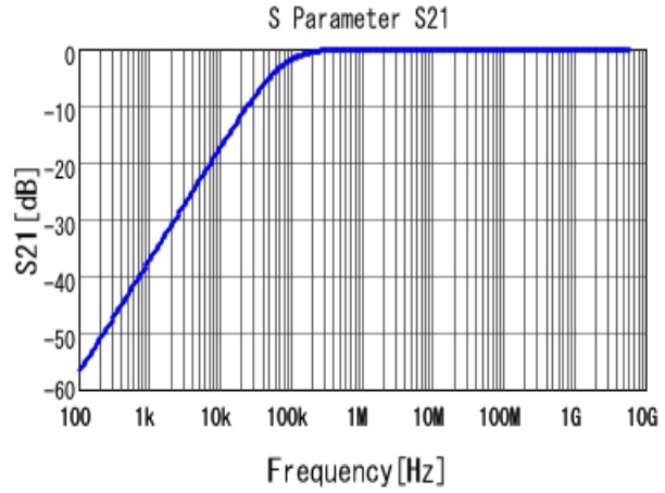
■ GRM033C80J223KE01 S21 DCOV, 25degC
