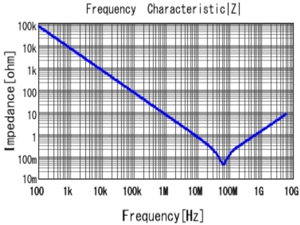
■ GRM033C80J223KE01 |Z| DCOV, 25degC
