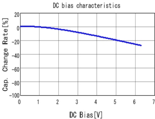
■ GRM033C80J223KE01 C-DC bias capchange, 25.0degC, AC0.
