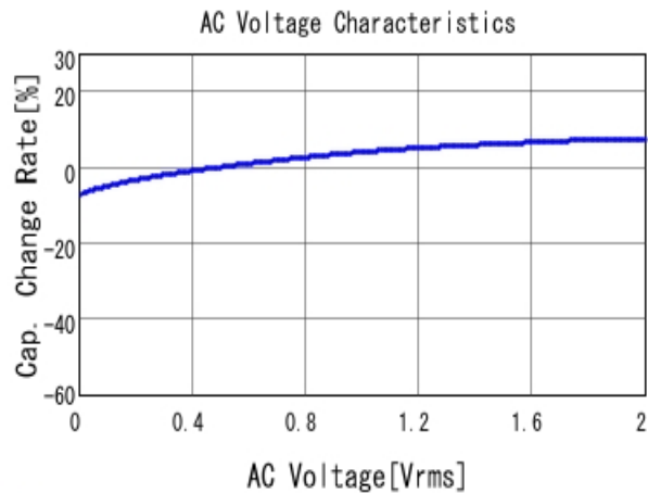
■ GRM033C80J223KE01 C-AC Voltage capchange, DCOV, 25.0d
