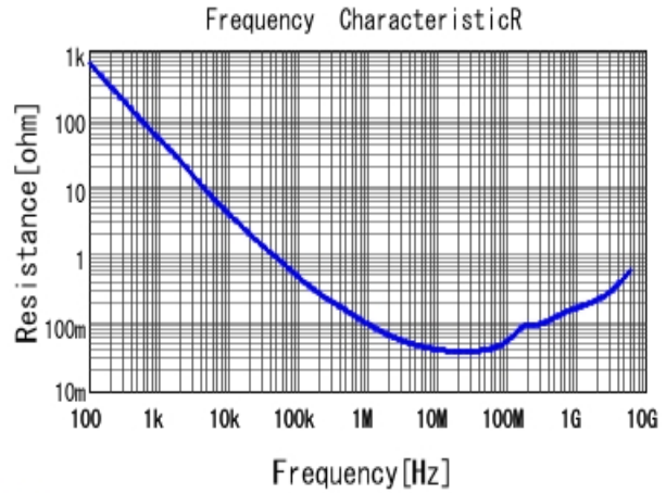
■ GRM033C80J223KE01 R DCOV, 25degC
