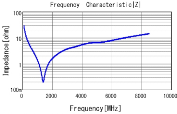
■ GRM0335C1H560JA01 |Z| DCOV, 25degC
