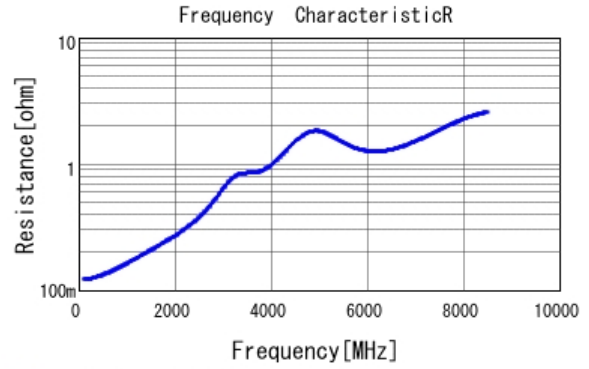
■ GRM0335C1H560JA01 R DCOV, 25degC
