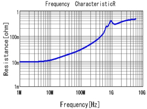
■ GRM0335C1E102JA01 R DCOV, 25degC
