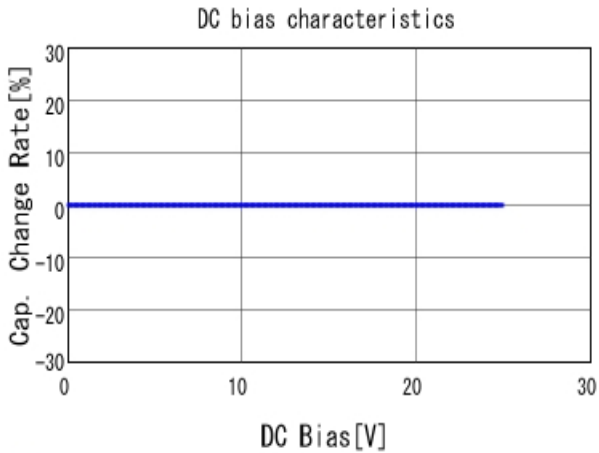
■ GRM0335C1E102JA01 C-DC bias capchange, 25.0degC, AC1V
