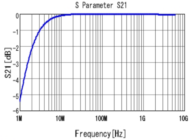
■ GRM0335C1E102JA01 S21 DCOV, 25degC
