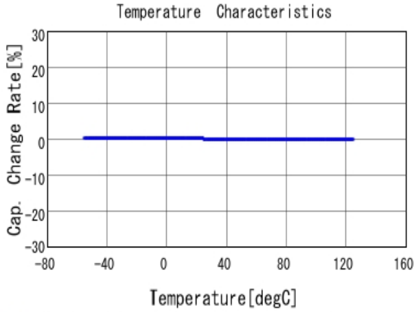
■ GRM0335C1E102JA01 C-Temp. capchange, DCOV, AC1Vrms
