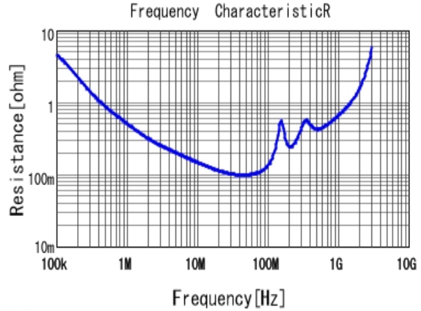
■ GR443DR73D472KW01 R DC0V, 25degC
