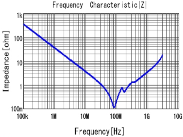
■ GR443DR73D472KW01 |Z| DC0V, 25degC
