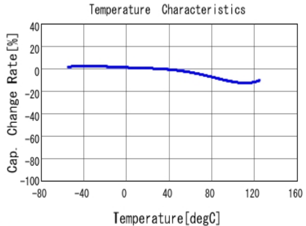
■ GR443DR73D472KW01 C-Temp. capchange, DC0V, AC1Vrms
