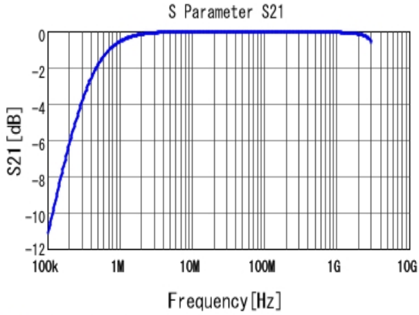
■ GR443DR73D472KW01 S21 DCOV, 25degC
