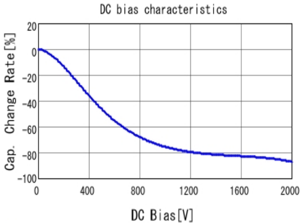
■ GR443DR73D472KW01 C-DC bias capchange, 25.0degC, AC1V
