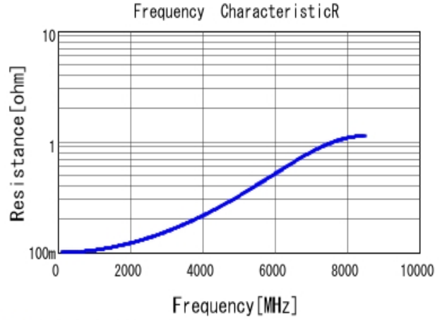
■ GJM1555C1H5R0BB01 R DC0V, 25degC
