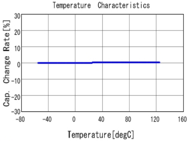
■ GJM1555C1H5R0BB01 C-Temp. capchange, DCOV, AC1Vrms
