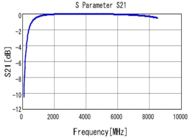
■ GJM1555C1H5R0BB01 S21 DCOV, 25degC
