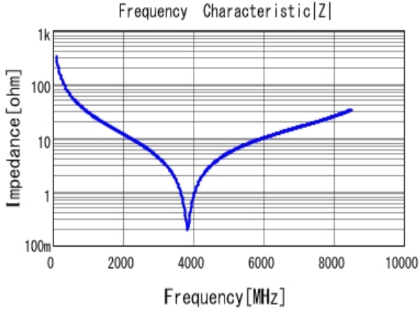
■ GJM1555C1H5R0BB01 |Z| DC0V, 25degC
