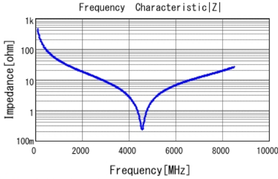
■ GJM1555C1H3R6WB01 |Z| DCOV, 25degC
