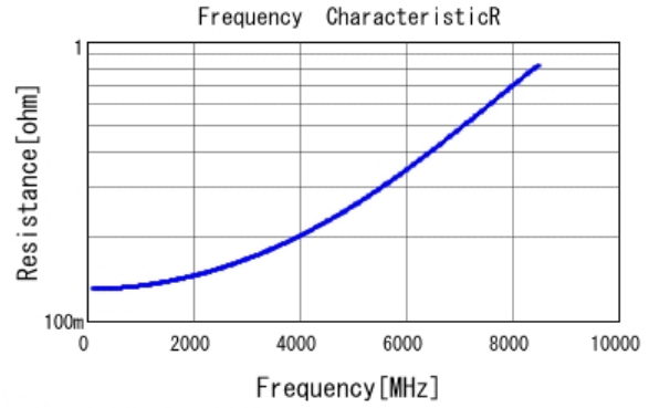
■ GJM1555C1H3R6WB01 R DCOV, 25degC
