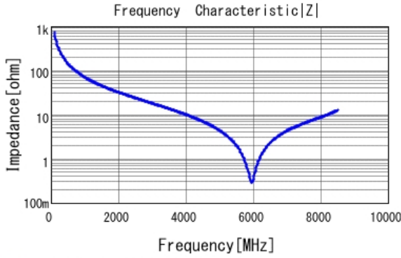
■ GJM1555C1H2R2CB01 |Z| DCOV, 25degC
