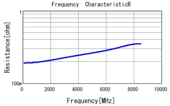
■ GJM1555C1H2R2CB01 R DCOV, 25degC
