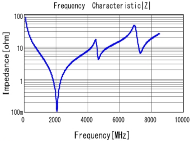
■ GJM1555C1H200GB01 |Z| DC0V, 25degC
