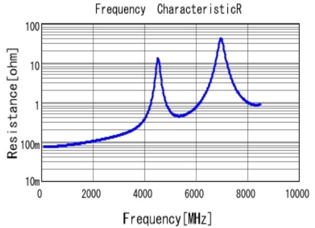
■ GJM1555C1H200GB01 R DC0V, 25degC
