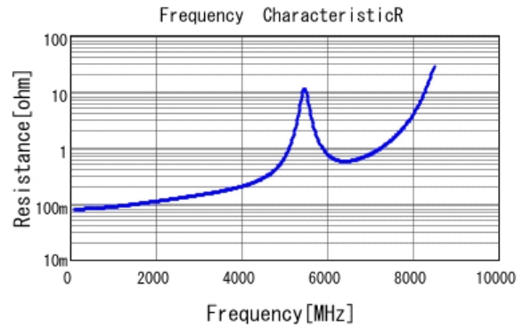
■ GJM1555C1H150GB01 R DC0V, 25degC
