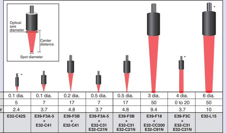
<Map of Spot Diameters and Center Distances> (Unit: mm)
