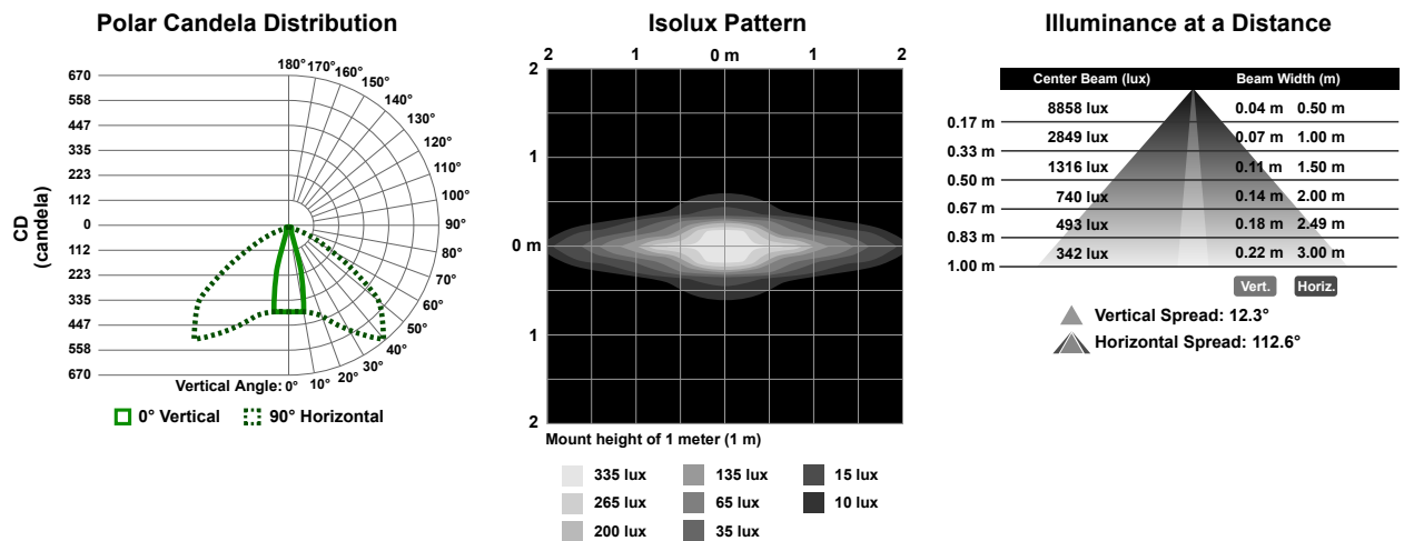
Figure 2. L25 Window
