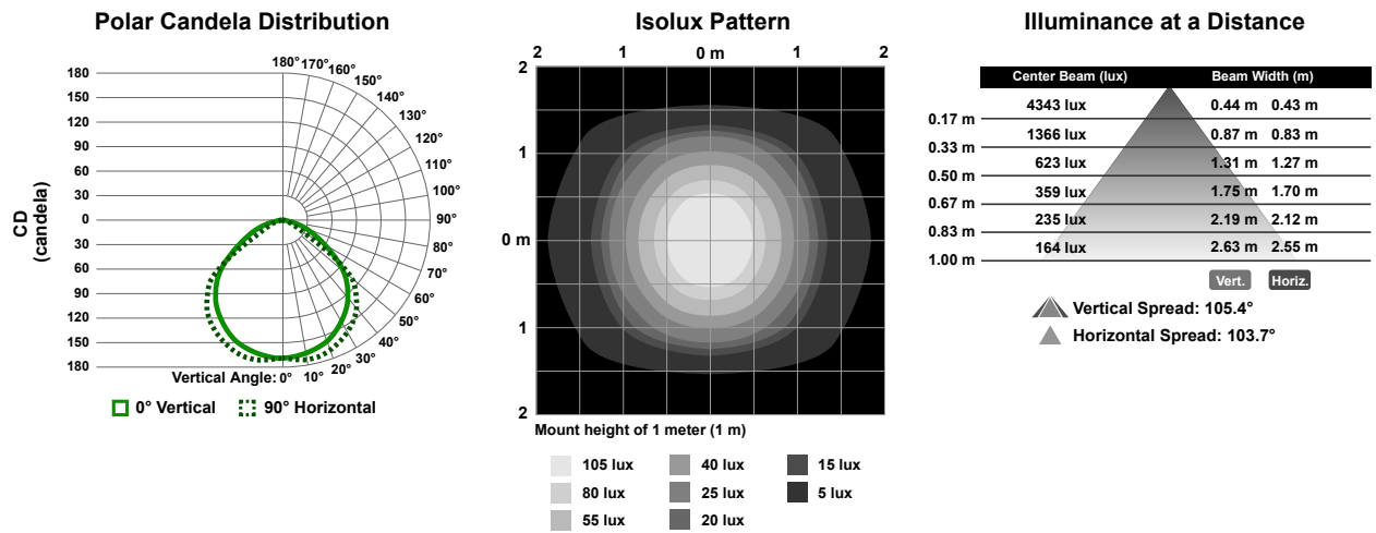
Figure 1. Clear Window
