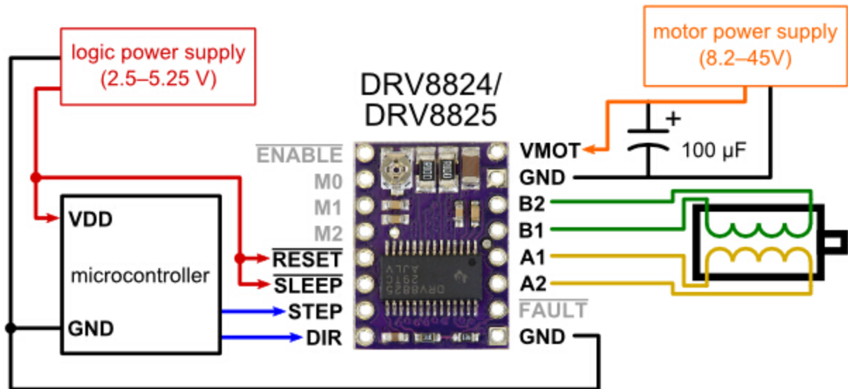
Minimal wiring diagram for connecting a microcontroller to a DRV8824/DRV8825 stepper motor driver carrier (full-step mode).
