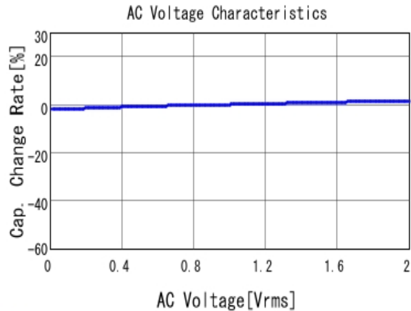
GCM155R71H471KA37 C-AC Voltage capchange, DCOV, 25.0d
