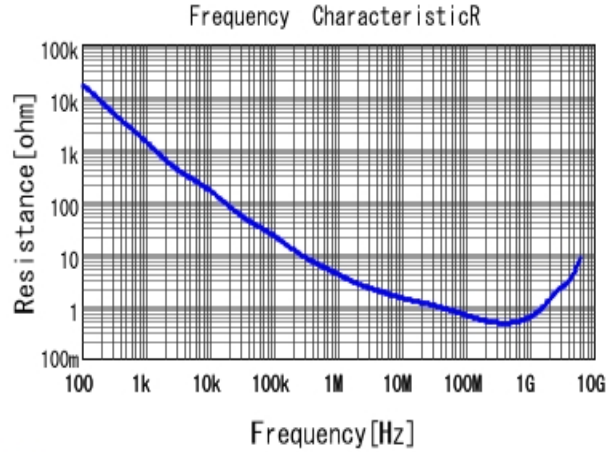
GCM155R71H471KA37 R DCOV, 25degC
