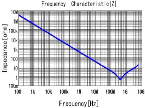
GCM155R71H471KA37 |Z| DCOV, 25degC
