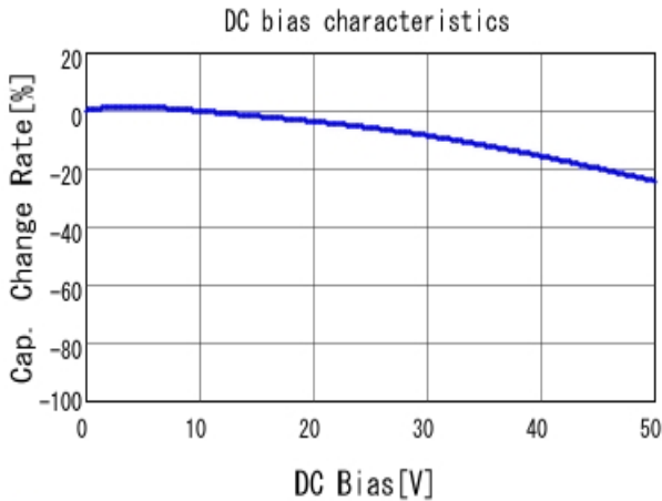
GCM155R71H471KA37 C-DC bias capchange, 25.0degC, AC1.
