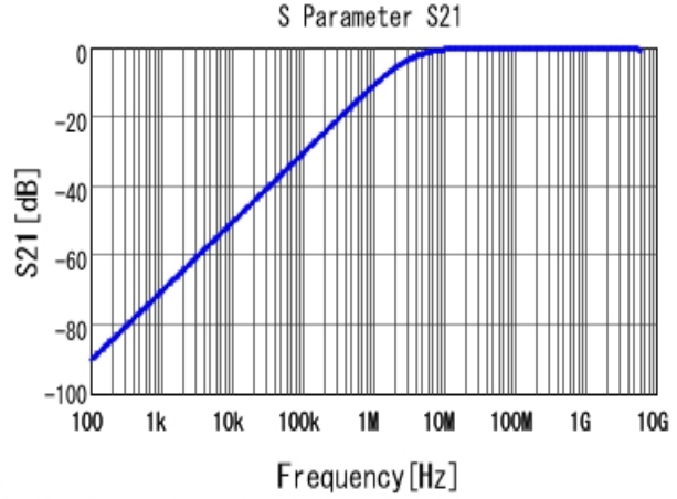
■ GCM155R71H471KA37 S21 DC0V, 25degC
