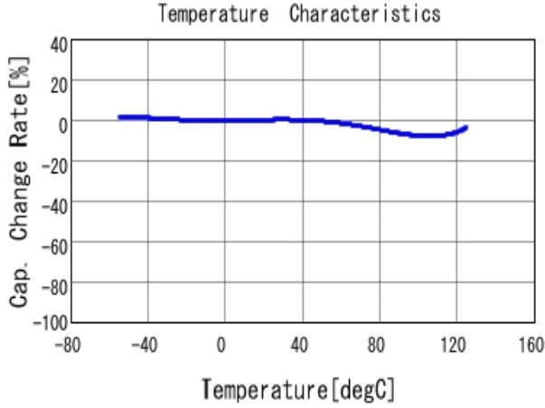
■ GCM155R71H471KA37 C-Temp. capchange, DC0.0V, AC1.0V rm
