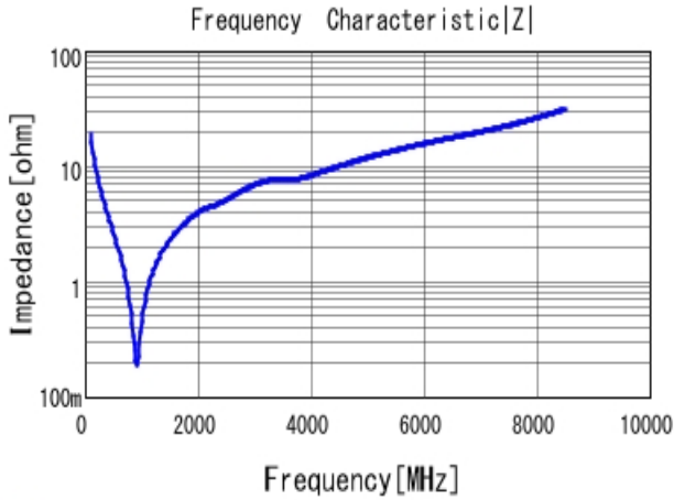
GCM1555C1H820JA16 |Z| DC0V, 25degC
