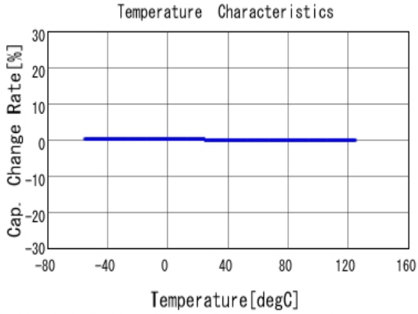
■ GCM1555C1H820JA16 C-Temp. capchange, DCOV, AC1Vrms
