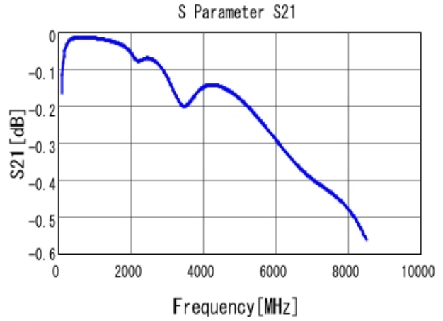
■ GCM1555C1H820JA16 S21 DCOV, 25degC
