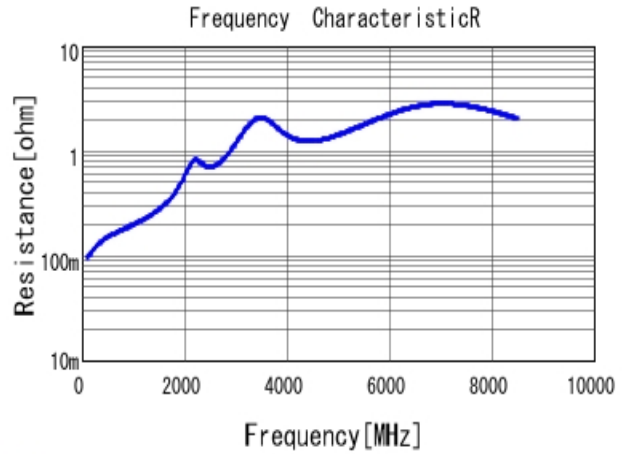
GCM1555C1H820JA16 R DC0V, 25degC
