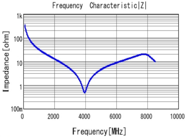
GCM1555C1H4R7CA16 |Z| DC0V, 25degC
