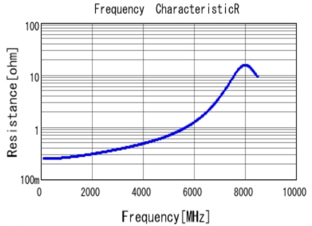
GCM1555C1H4R7CA16 R DC0V, 25degC
