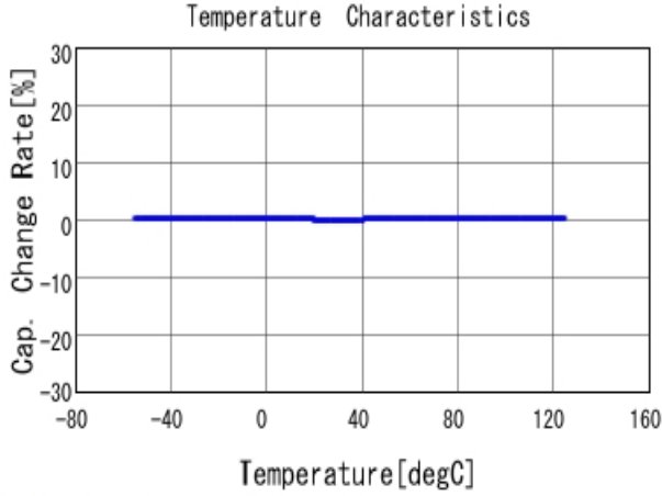
■ GCM1555C1H4R7CA16 C-Temp. capchange, DCOV, AC1Vrms
