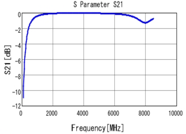
■ GCM1555C1H4R7CA16 S21 DCOV, 25degC
