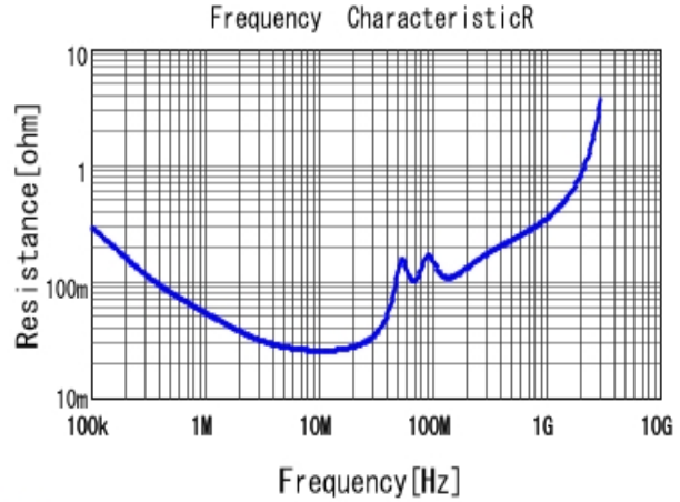
■ GCJ43DR72J473KXJ1 R DC0V, 25degC
