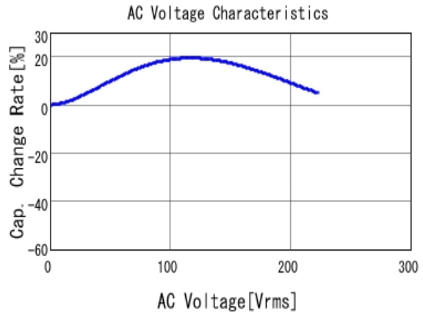
■ GCJ43DR72J473KXJ1 C-AC Voltage capchange, DC0V, 25.0d
