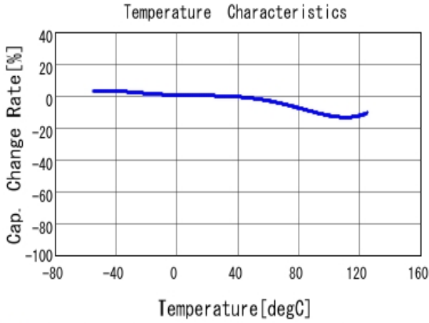
GCJ43DR72J473KXJ1 C-Temp. capchange, DCOV, AC1Vrms
