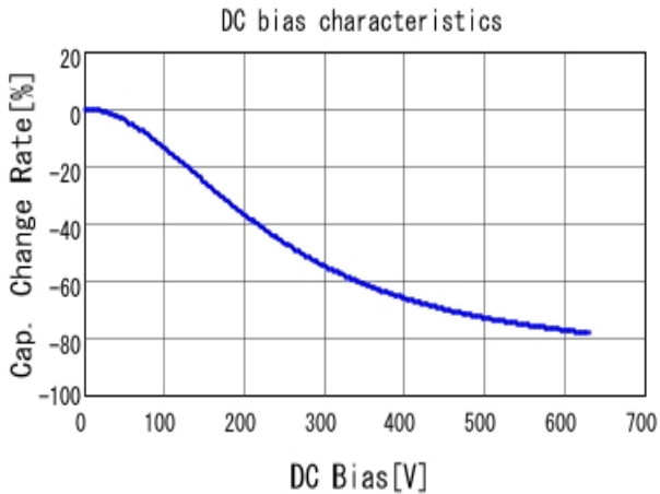
■ GCJ43DR72J473KXJ1 C-DC bias capchange, 25.0degC, AC1V
