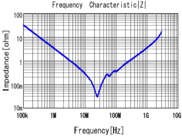
■ GCJ43DR72J473KXJ1 |Z| DC0V, 25degC
