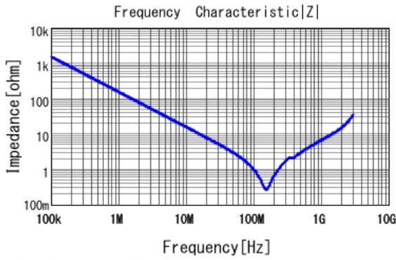
■ GA352QR7GF102KW01 |Z| DCOV, 25degC
