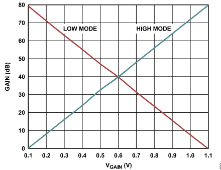
Figure 44. Two Gain Control Modes of the AD8338
