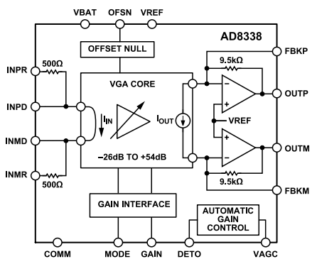
Figure 39. Block Schematic
