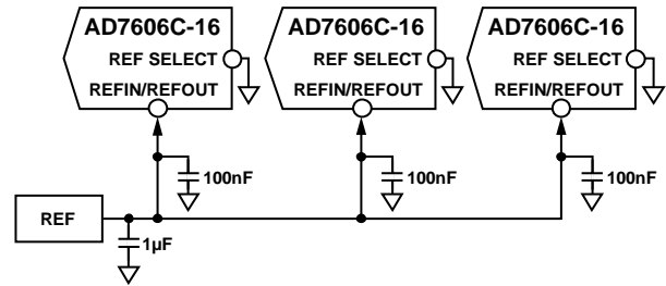
Figure 84. Single External Reference Driving Multiple AD7606C-16 REFIN/REFOUT Pins
