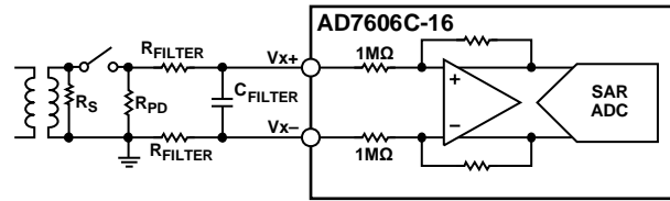
Figure 95. Analog Front End with R_{PD}
