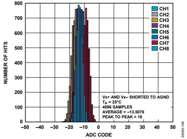
Figure 55. Histogram of Codes, ±10 V Single-Ended Range
