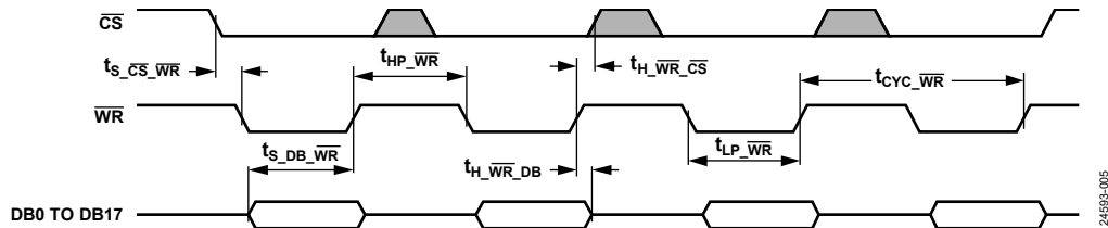
Figure 5. Parallel Mode Write Operation
