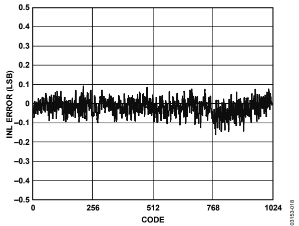
Figure 18. Typical INL for the AD7441
