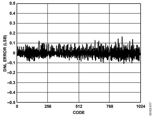
Figure 17. Typical DNL for the AD7441
