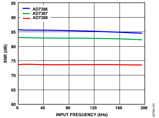
Figure 23. SNR vs. Input Frequency
