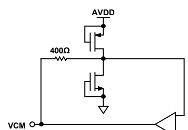
Figure 28. Equivalent VCM Circuit
