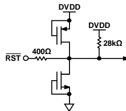
Figure 26. \overline{RST} Equivalent Circuit
