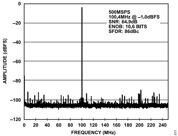
Figure 11. 16k Point Single-Tone FFT; 500 MSPS, 100.4 MHz
