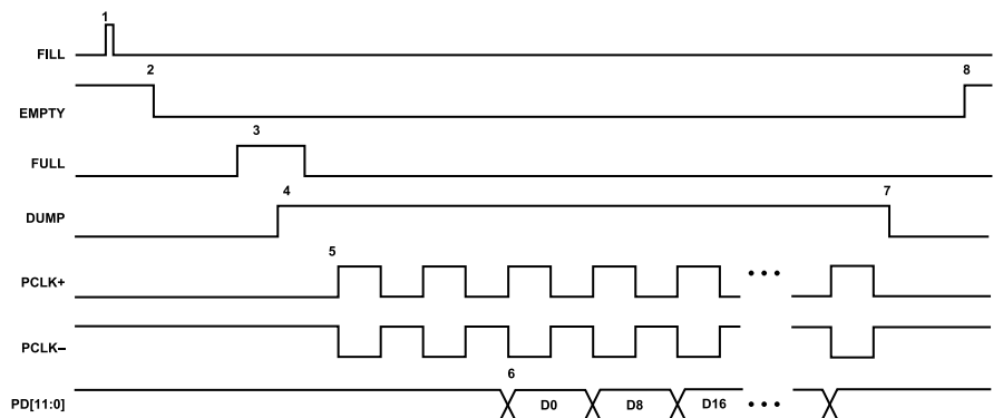
Figure 40. Parallel Mode Transaction Diagram
