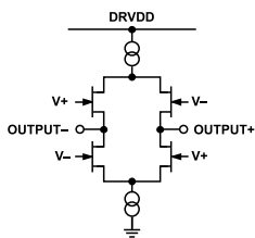
Figure 30. LVDS Outputs (PDOR±, PD[5:0]±, PCLK±)
