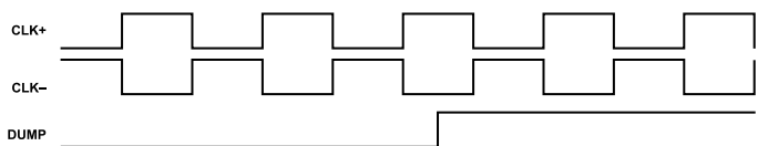
Figure 38. FIFO DUMP Timing
