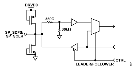
Figure 34. Equivalent SP_SDFS and SP_SCLK Circuit
