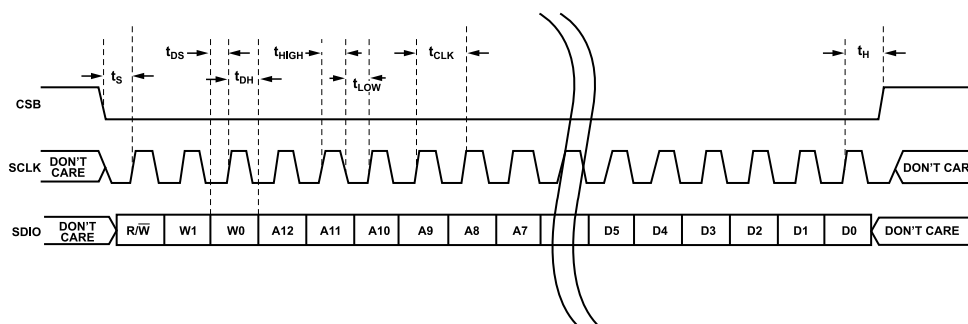
Figure 43. Serial Port Interface Timing Diagram
