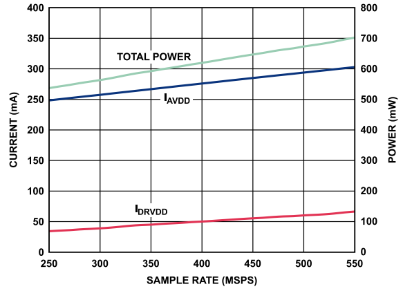
Figure 25. Current and Power vs. Sample Rate
