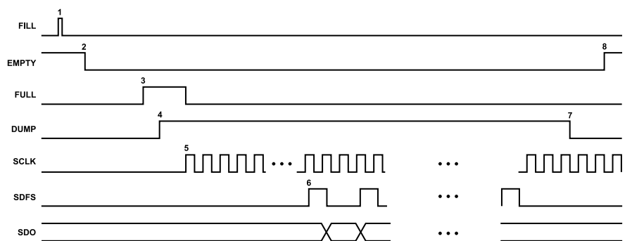
Figure 39. SPORT Leader Mode Transaction Diagram
