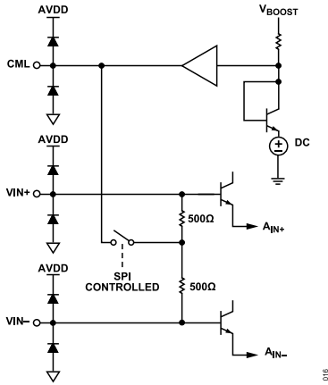
Figure 26. DC Equivalent Analog Input Circuit
