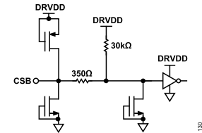
Figure 32. Equivalent CSB Input Circuit
