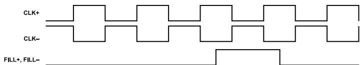
Figure 37. FIFO Fill Timing
