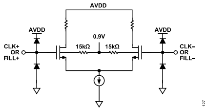
Figure 28. Equivalent CLK± and FILL± Input Circuit
