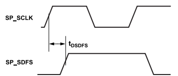
Figure 4. SP_SDFS Propagation Delay
