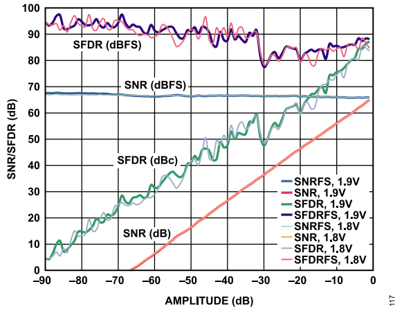
Figure 17. SNR/SFDR vs. Input Amplitude; 500 MSPS, 140.3 MHz
