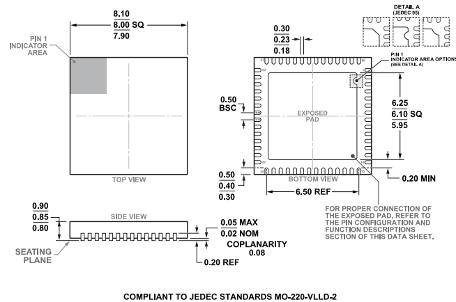
COMPLIANT TO JEDEC STANDARDS MO-220-VLLD-2 Figure 44. 56-Lead Lead Frame Chip Scale Package [LFCSP] 8 mm x 8 mm Body and 0.85 mm Package Height (CP-56-22) Dimensions shown in millimeters
