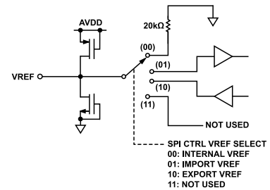
Figure 35. Equivalent VREF Circuit
