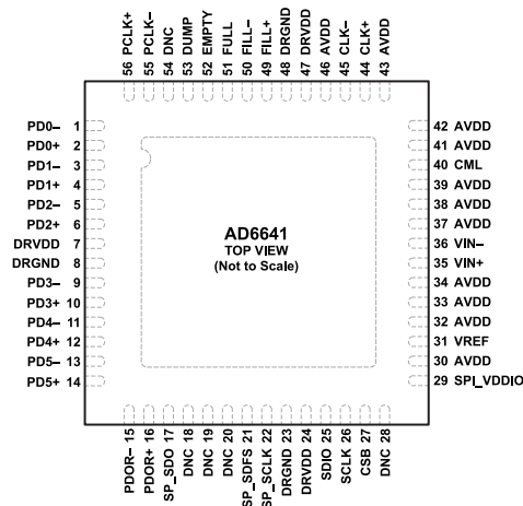
Figure 8. Pin Configuration for DDR LVDS Mode
