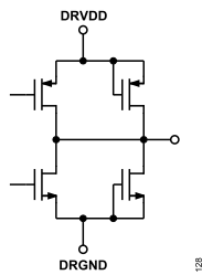
Figure 29. Equivalent PD[11:0], FULL, EMPTY, PCLK±, and SP_SDO Output Circuit
