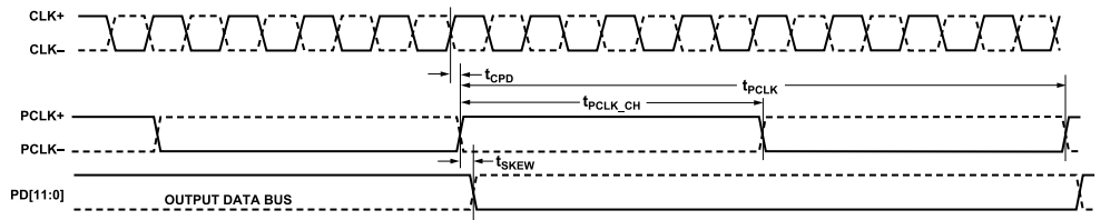
Figure 3. Parallel CMOS Mode Output Interface Timing
