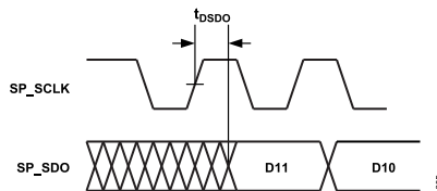
Figure 5. SP_SDO Propagation Delay
