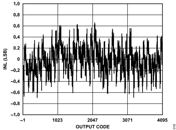
Figure 18. INL; 500 MSPS
