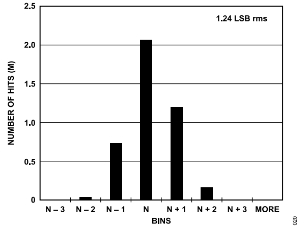
Figure 20. Grounded Input Histogram; 500 MSPS
