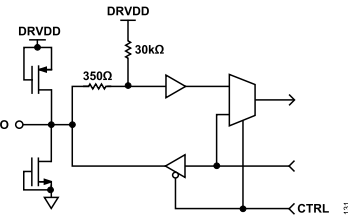
Figure 33. Equivalent SDIO Circuit
