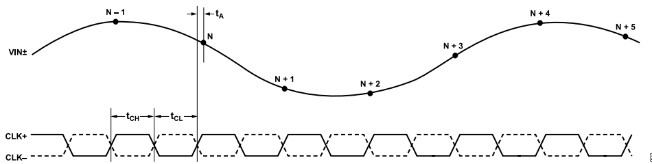
Figure 2. Input Interface Timing
