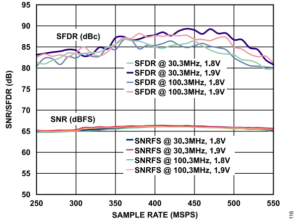
Figure 16. SNR/SFDR vs. Sample Rate and Supply
