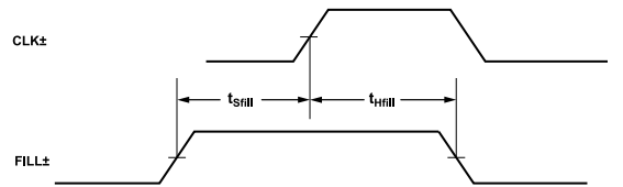
Figure 7. FILL± Setup and Hold Times
