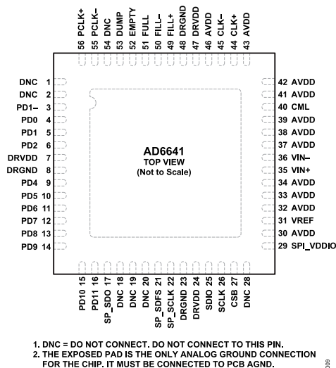
Figure 9. Pin Configuration for Parallel CMOS Mode
