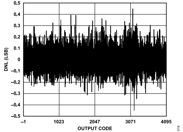
Figure 19. DNL; 500 MSPS
