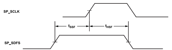
Figure 6. Follower Mode SP_SDFS Setup/Hold Time
