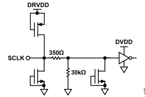
Figure 31. Equivalent SCLK Input Circuit
