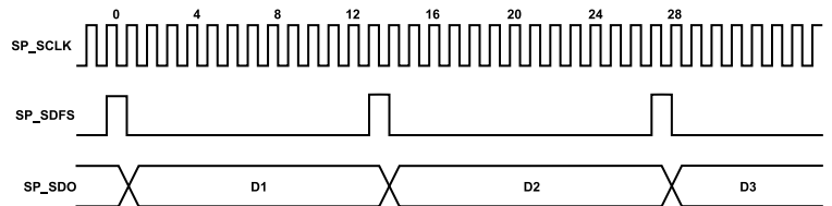
Figure 41. Data Output in Serial Bus Leader Mode
