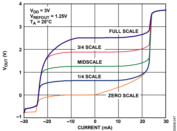
Figure 36. AD56x4R-3 Source and Sink Capability
