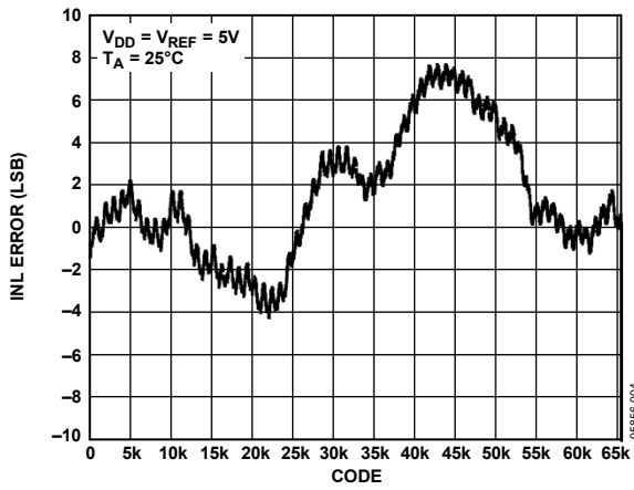
Figure 5. AD5664R INL, External Reference
