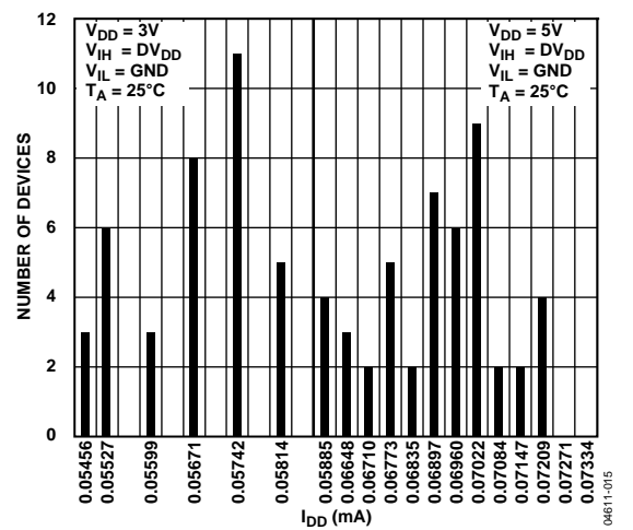
Figure 16. I_{DD} Histogram (3 V/5 V)
