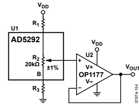
Figure 72. Optimizing Resolution
