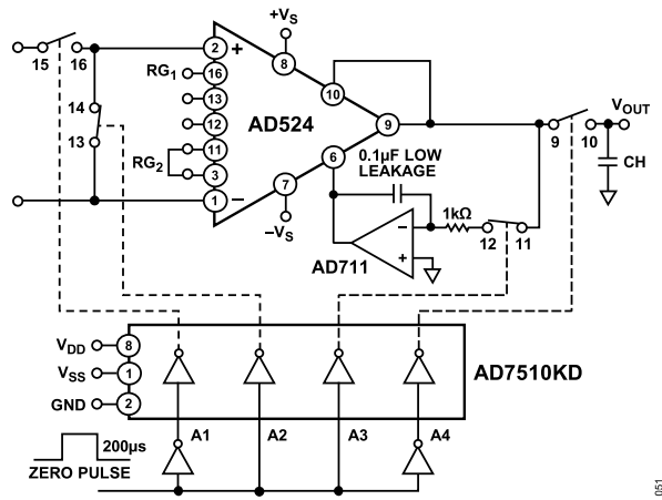
Figure 51. Auto-Zero Circuit
