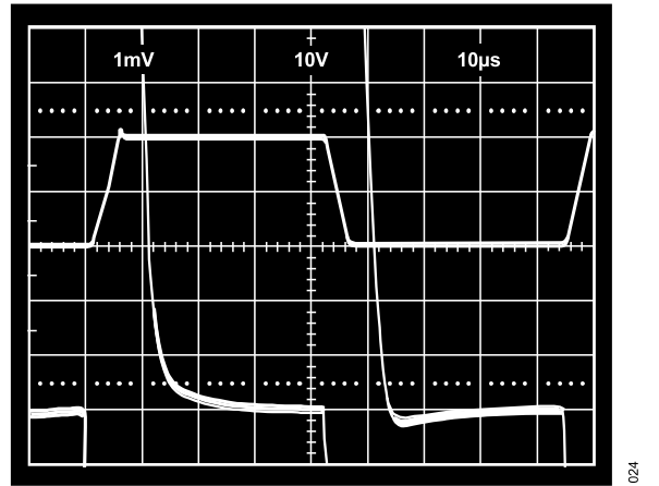
Figure 27. Large Signal Pulse Response and Settling Time, Gain = 10
