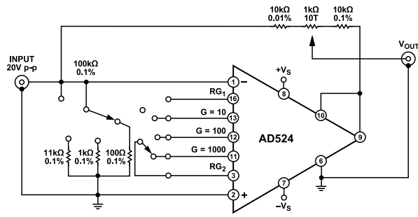
Figure 31. Settling Time Test Circuit
