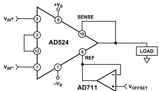
Figure 45. Use of Reference Terminal to Provide Output Offset
