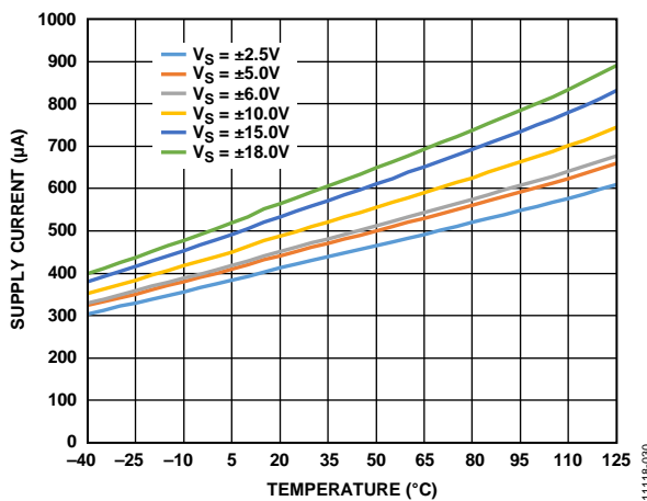
Figure 32. Supply Current vs. Temperature
