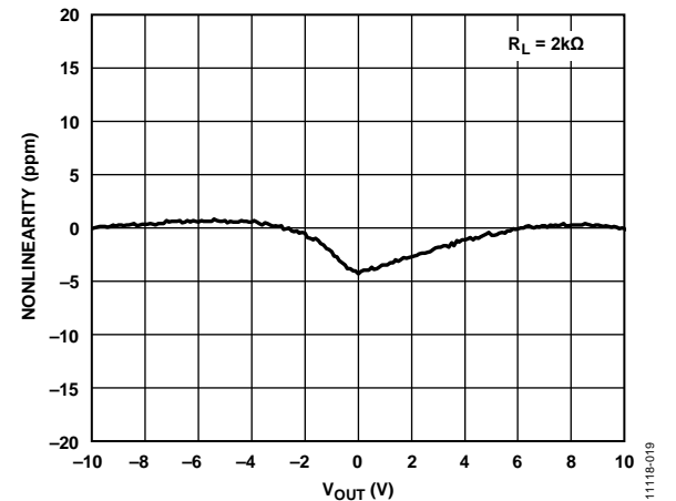
Figure 22. Gain Nonlinearity
