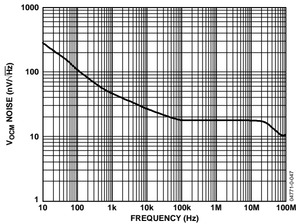
Figure 33. V_{OCM} Voltage Noise vs. Frequency
