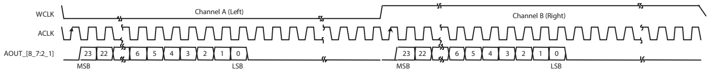
Figure 4-42: I 2 S Audio Output Format
