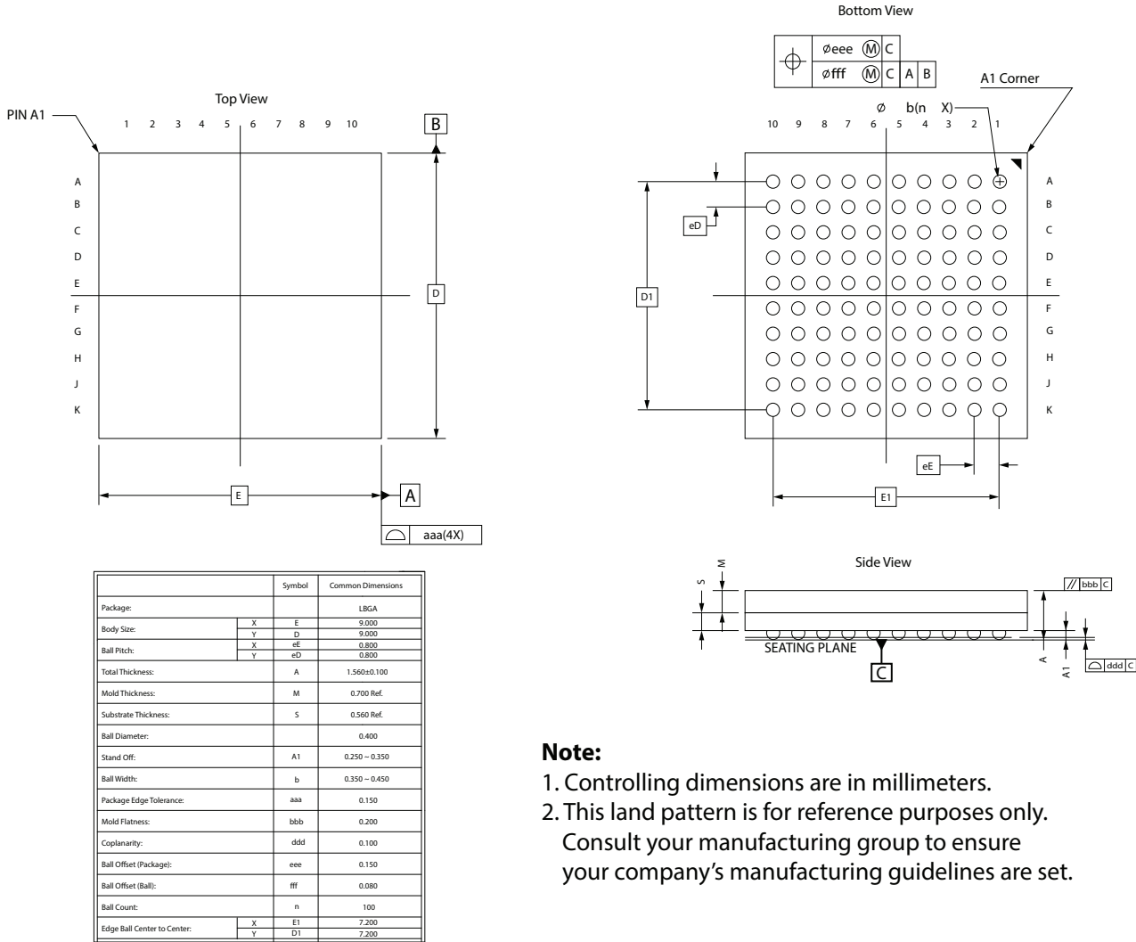
Figure 8-1: Package Dimensions
