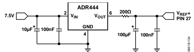
Figure 54. Reference Connection
