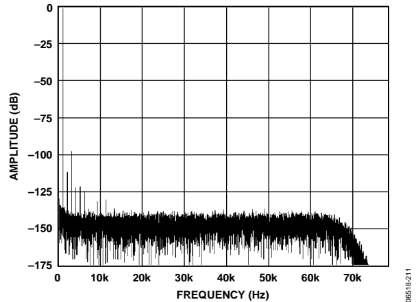
Figure 10. Low Power Mode, FFT, 1 kHz, -0.5 dB Input Tone, 128\times Decimation Rate
